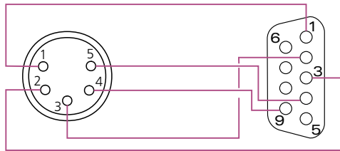
VCA500 Female XLR 5 points plug SNA50-2 et SNA50-2 live Female Sub-D 9 points plug
